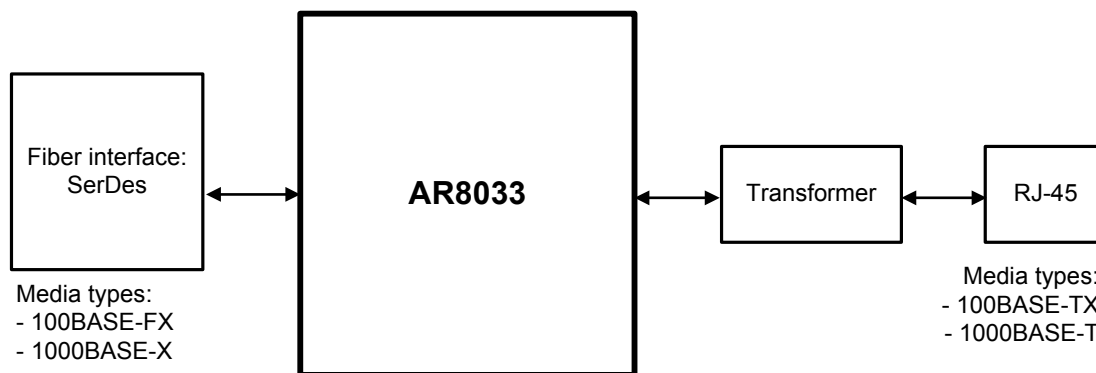
Figure 3-3 Media converter operating mode
