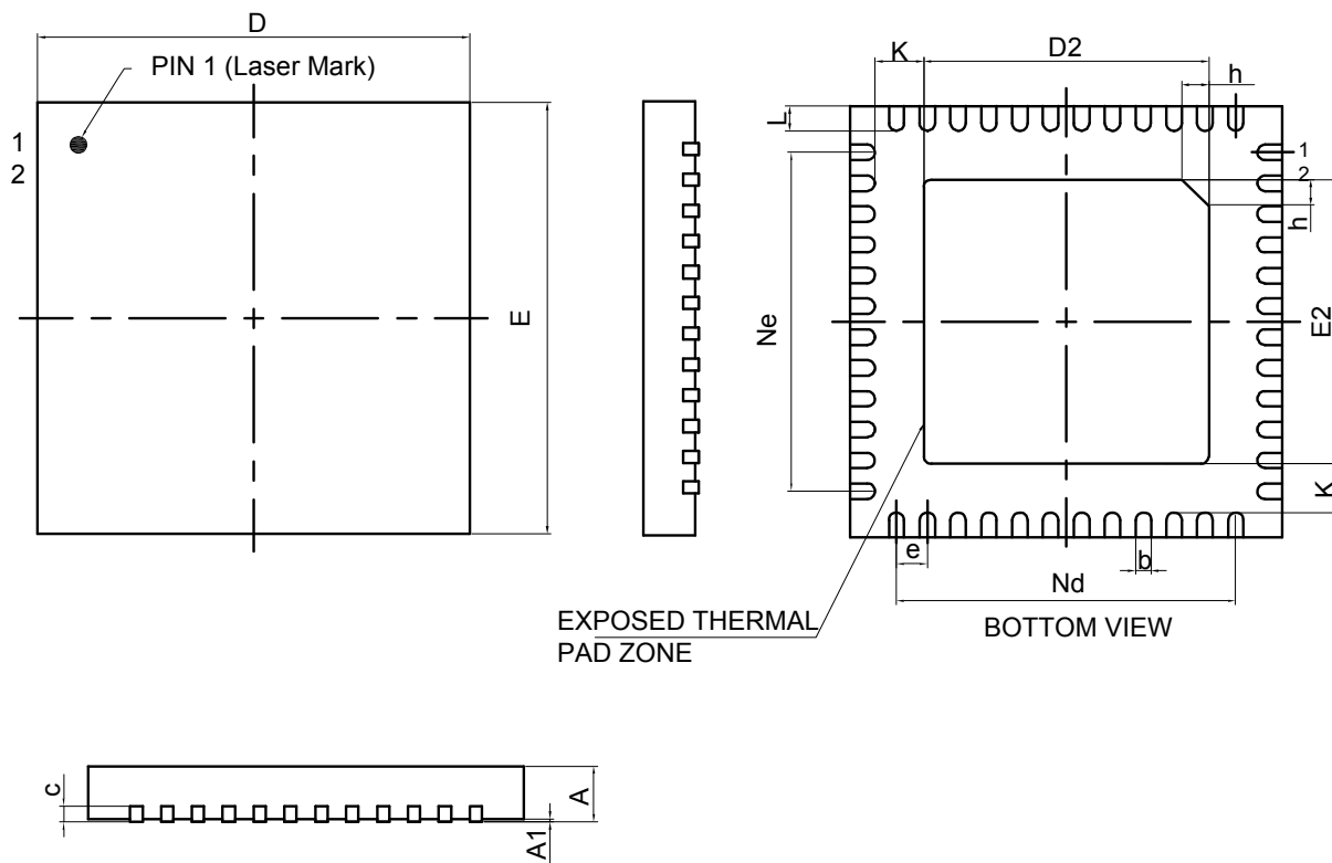
Figure 6-1 Packag view
