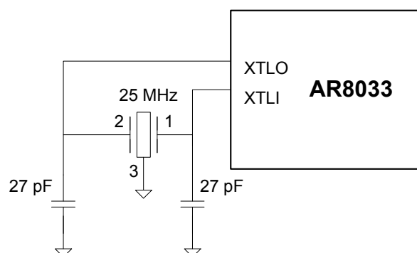
Figure 4-4 External crystal
