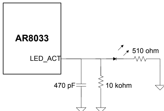
Figure 3-9 Reference design for LED, active high
