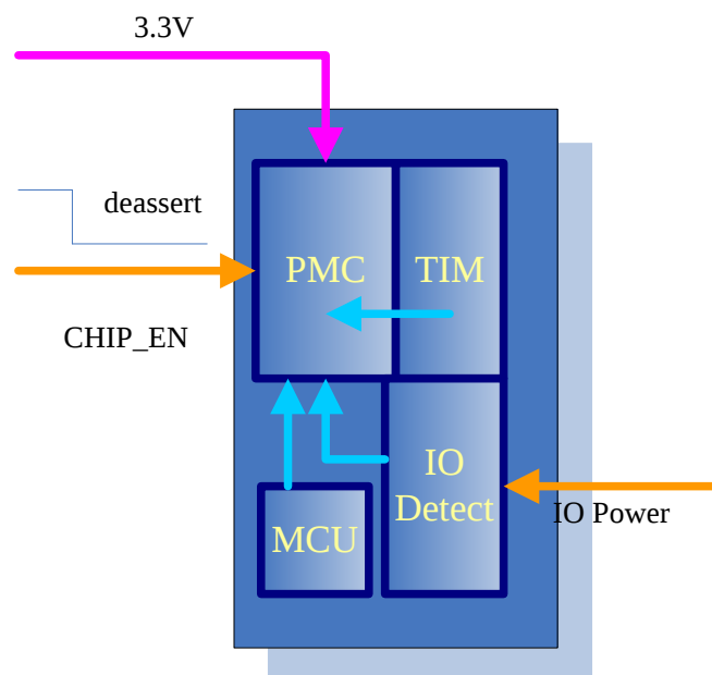
Figure 9 Shutdown Mode
